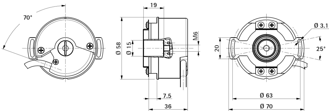
Figure 1 - CB59 encumbrance sizes
