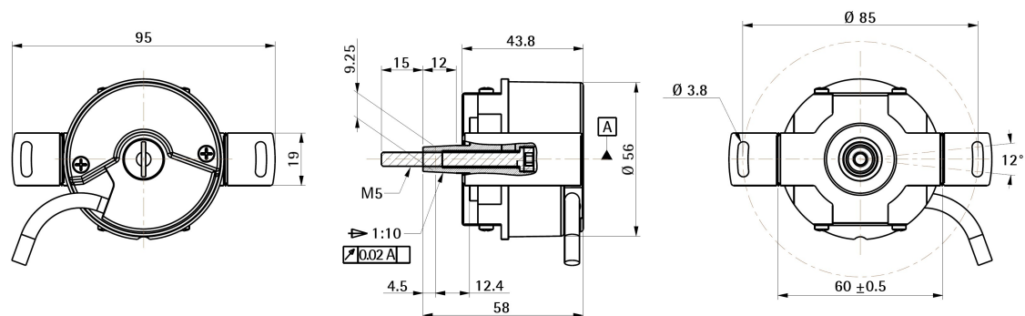
Figure 8 - CB62 encumbrance sizes (B order code)
