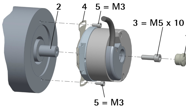
Figure 2 - Mounting of CB59 encoder
