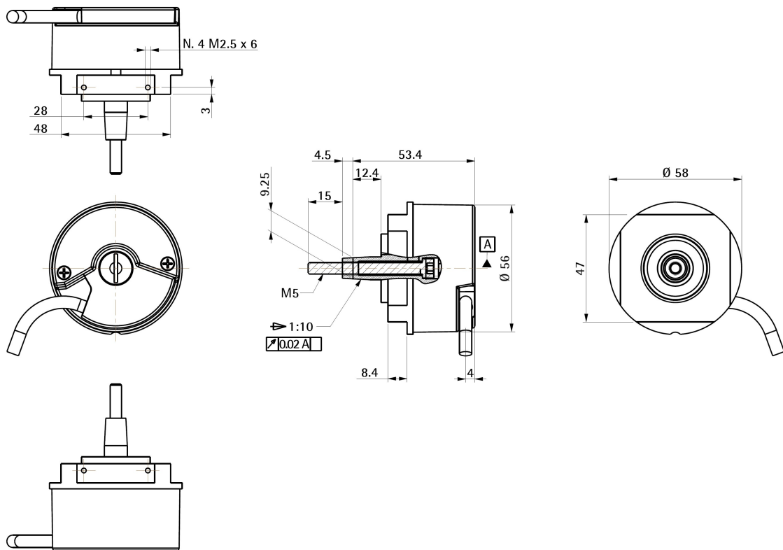
Figure 7 - CB62 encumbrance sizes (A order code)
