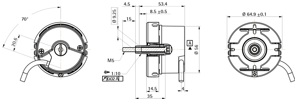
Figure 4 - CB62 encumbrance sizes (standard version)
