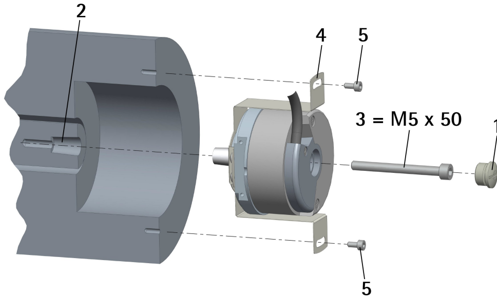
Figure 11 - Example with B type fixing plate
