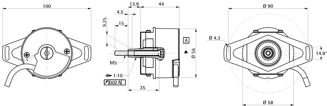
Figure 9 - CB62 encumbrance sizes (D order code)
