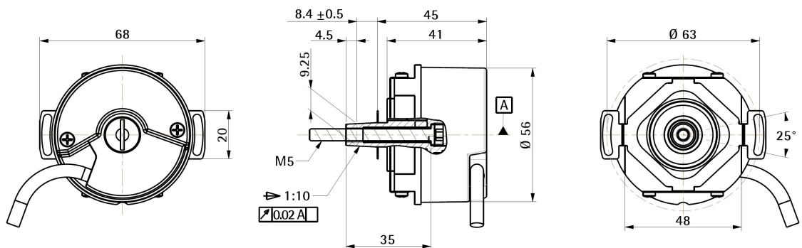
Figure 10 - CB62 encumbrance sizes (E order code)
